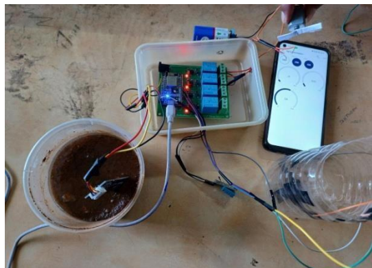
Figure 7: Before connection
